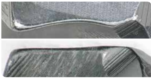
After drilling 900 holes
