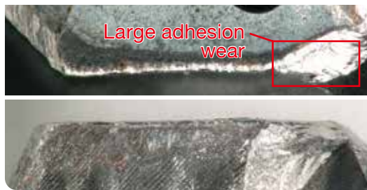
After drilling 3,840 holes
